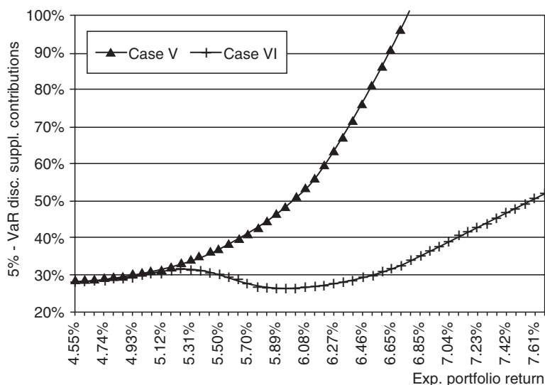
Figure 11-2. Worst-case plan costs vs. asset allocation.
