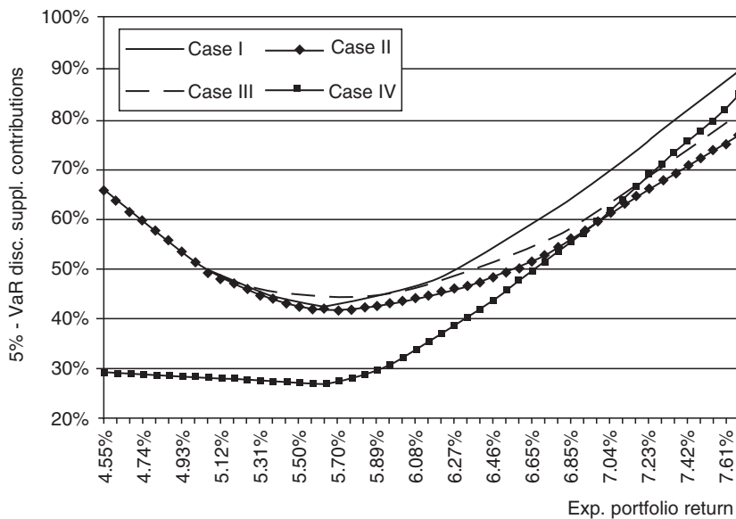
Figure 11-1. Worst-case plan costs vs. asset allocation.
