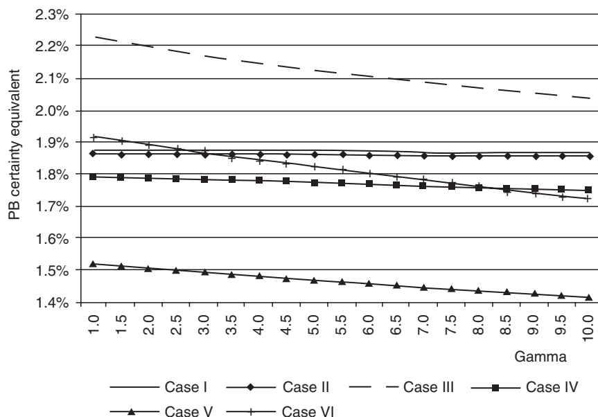
Figure 11-3. Certainty equivalents of pension benefit factors for different plan designs with sponsor's optimal asset allocation.
