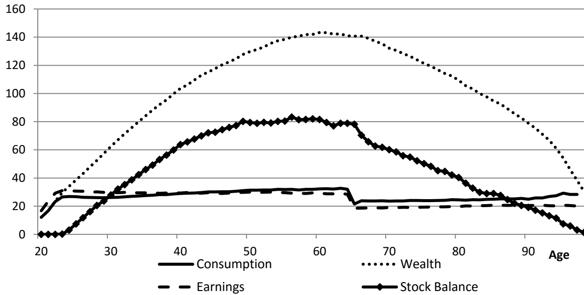
Figure 6.1. Life cycle profiles of key variables from a baseline model.
