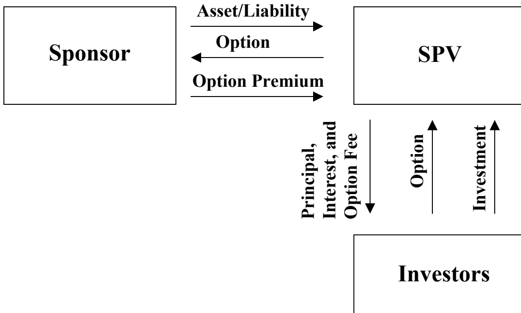
Figure 2. Credit-linked Note.
